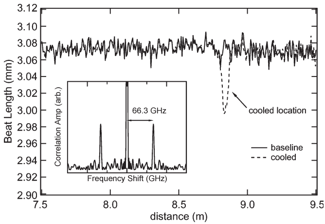
Fig. 5. Spatial variation of the beat length of the PM fiber as calculated from the frequency shift of the autocorrelation function as shown in the inset graph. Two measurements of the fiber were made; in the second measurement, a piece of ice was placed on the fiber to induce local cooling, which decreased the beat length locally. Note that the variability outside the cooled segment is highly repeatable.
